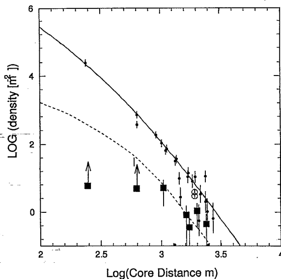
FIG. 2. The lateral distribution of charged particle (closed circles) and muons (shaded squares). The large open circle is that measured by a detector for arrival time distribution. The expected lateral distribution of charged particles is shown by a solid line and that of muons by a dotted line.
