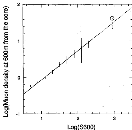
FIG. 3. \rho_\mu(600) vs S_0(600) relation. An open circle is the estimated value of the present event, and filled circles are average values for each bin determined by the AGASA experiment.
