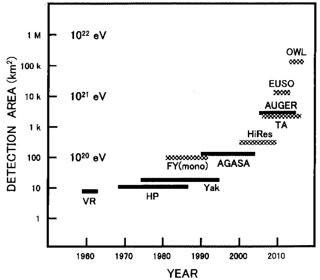
Fig. 1. The increase of the covered ground area with time for the past, present and future EHECR detectors. Approximate energy limit of the investigation is also shown in the ordinate.
