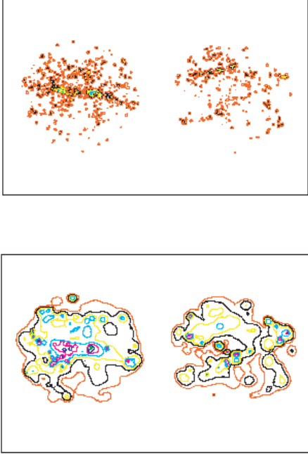
Fig. 2. (a) upper panel: Same with Figure 1b, but for E \geq 10^{20.0} eV. (b) lower panel: Same with Figure 2a, but for B = 100 nG.
