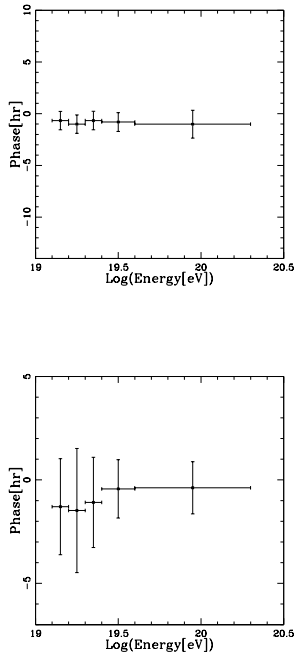
Fig. 13. (a) upper panel: same with Figure 12a, but for the phase of the first harmonics. (b) lower panel: same with Figure 13a, but for the second harmonics.
