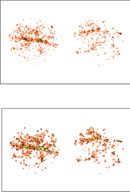
Fig. 3. (a) upper panel: Same with Figure 2a, but for l_c = 1 Mpc (b) lower panel: Same with Figure 2a, but for l_c = 40 Mpc
