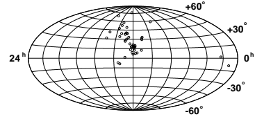
Fig. 4. Arrival directions of UHECRs above 4 \times 10^{19} eV in equatorial coordinates for the case of B = 10 nG and l_c = 1 Mpc. The number of events is chosen to be 47 in order to compare our results with the AGASA data (Hayashida 1999). The arrival directions of UHECRs are restricted in the range -15^\circ \leq b \leq 80^\circ in order to compare our results with the AGASA data. Clusters which mean the small-scale anisotropy of UHECRs can be found clearly.
