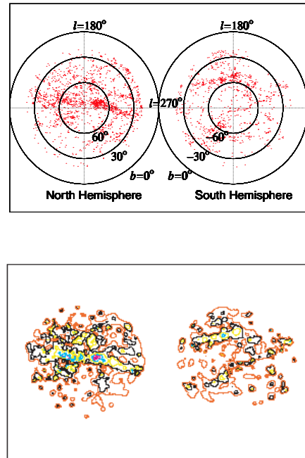
Fig. 1. (a) upper panel: angular distribution of galaxies in Optical Redshift Survey (ORS) data within 40Mpc. (b) lower panel: distribution of arrival directions of UHECRs in the case of B = 10 nG, l_c = 10 Mpc, H_0 = 75 km/s/Mpc, and E \geq 10^{19.5} eV. Galactic coordinate is used and left parts correspond to the north galactic hemisphere. The resolution of the image is set to be 1^\circ \times 1^\circ . The inter-contour interval is 0.5 in the logarithm to base 10 of the integral flux per solid angle.
