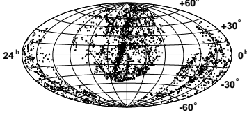
Fig. 5. Angular distribution of galaxies in ORS data within 40Mpc in equatorial coordinate. It is noted that this database does not contain any data within |b| \leq 20^\circ .
