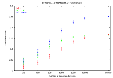
Fig. 9. Correlation values for the case of B = 10 nG, l_c = 10 Mpc and H_0 = 75.0 km/s/Mpc indicating the influence of the selected energy range. n = 0 , n = 1 , and n = 2 denote E \geq 10^{19.5}\text{eV} , E \geq 10^{20.0}\text{eV} , and E \geq 10^{21.0}\text{eV} , respectively. It is noted that the present observed number ( N ) of UHECRs of order 10^1 is too small to estimate the final correlation values. When N is close to the order of 10^3 - 10^4 , the correlation values begin to converge.
