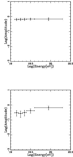
Fig. 12. (a) upper panel: amplitude of the first harmonics in galactic longitude in each energy bin for the case of B = 10 nG and l_c = 1 Mpc. N is chosen to be 47 in the energy range ( 4 \times 10^{19} - 2 \times 10^{20} eV) in order to compare our results with the AGASA data (Hayashida 1999). The number of data samples is set to be 1000 in order to obtain the mean value and the standard deviation in every bin. (b) lower panel: same with Figure 12a, but for the second harmonics.
