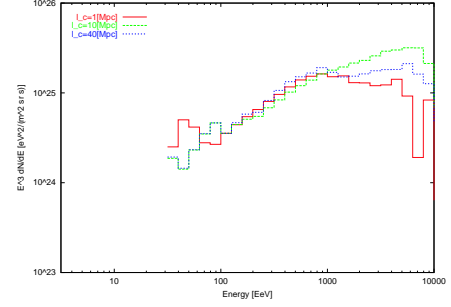
Fig. 8. Calculated energy spectra of UHECRs. The parameters are set to be B = 10 nG and H_0 = 75 km/s/Mpc. The cases of l_c = 1, 10 and 40 Mpc are shown respectively. The energy spectra are normalized to the AGASA data (Hayashida et al. 1999) at E = 100 EeV.
