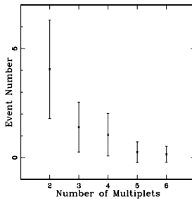
Fig. 7. Number of clusters such as doublets and triplets within a separation angle of 2.5^\circ in a data sample which contains 47 events, whose energies are above 4 \times 10^{19} eV. The number of data samples is set to be 20 in order to obtain the mean values.
